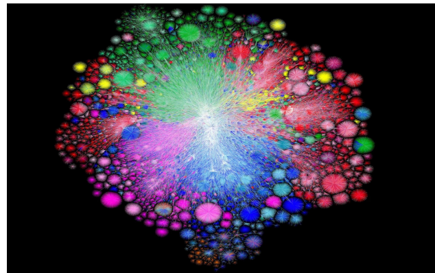
Internet, 2022
